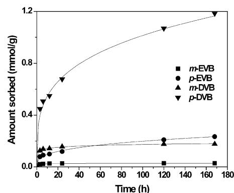
Figure 4. Liquid sorption profiles for the DVB mixture in dehydrated Mg-CUK-1 recorded at 25 °C as a function of sorption time.
